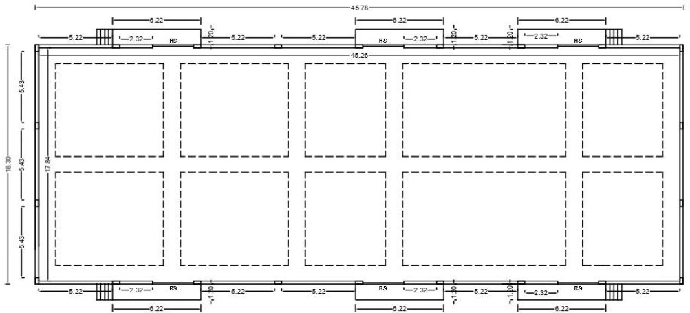
PLAN FOR 1448 MT WAREHOUSE SCALE 1:100
